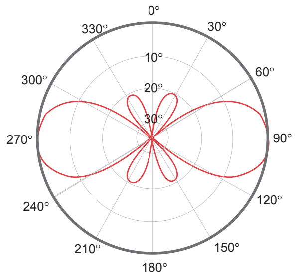
Antenna Radiation Pattern
